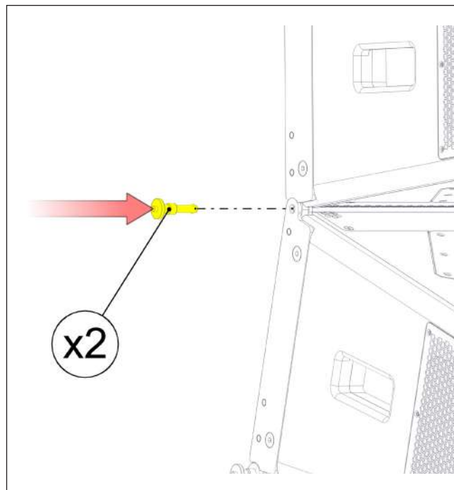
Fig. 21 - attach second block
